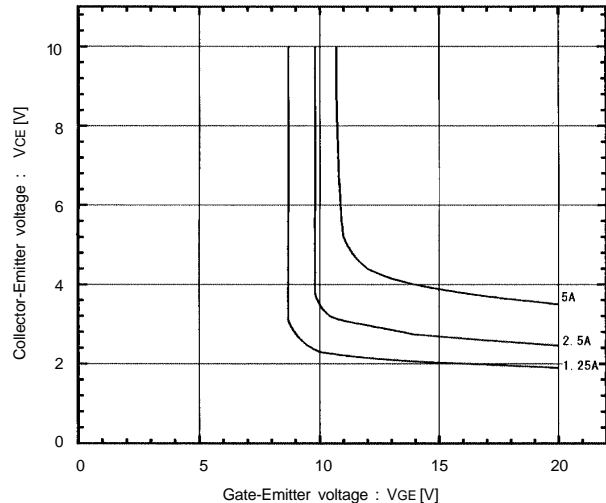
Collector-Emmitter vs. Gate-Emmitter voltage T j =125°C
