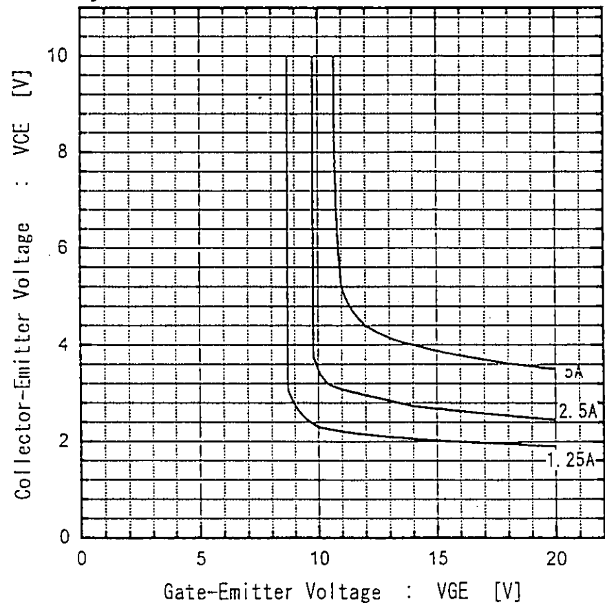
Collector-Emmitter Voltage vs Gate-Emmitter Voltage Tj=125°C
