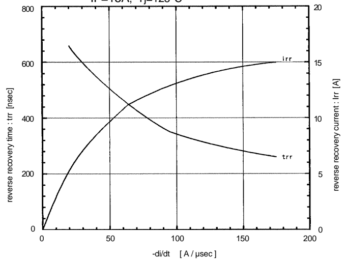
Reverse recovery time characteristics vs. -di/dt I_F=15A, T_j=125^{\circ}C
