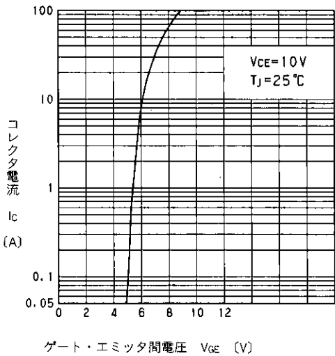
伝達特性(標準値) Typical Transfer Characteristics
