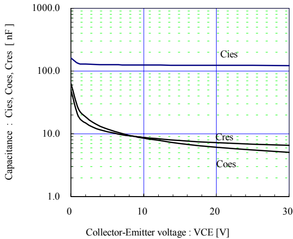
Capacitance vs. Collector-Emittor voltage (typ.) V_{GE}=0V, f = 1\text{MHz}, T_j = 25^\circ\text{C}
