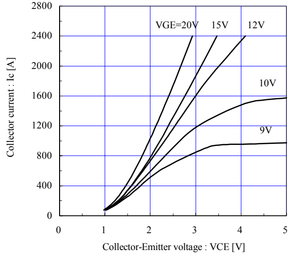
Collector current vs. Collector-Emittor voltage (typ.) T_j = 125^\circ\text{C}, \text{sense terminal}
