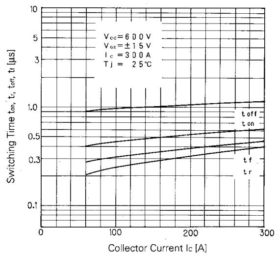
Switching Time
