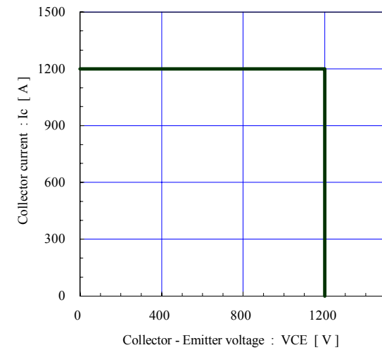
Reverse bias safe operating area (max.) +V_{GE}=15V, -V_{GE} \leq 15V, R_g \geq 0.6\Omega, T_j \leq 125^\circ C
