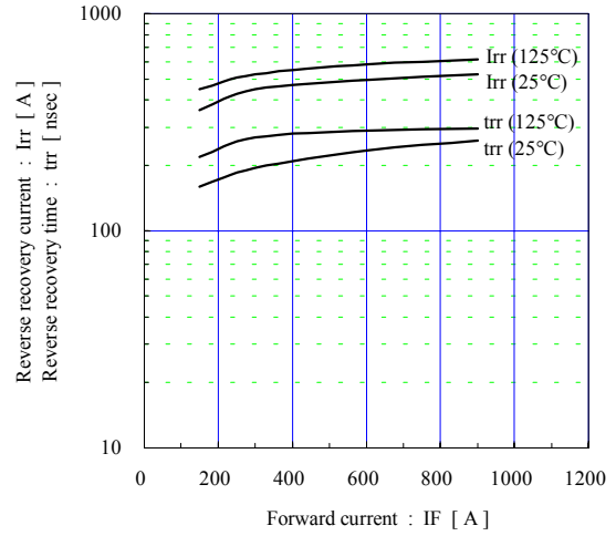
Reverse recovery characteristics (typ.) Vcc=600V, VGE=±15V, Rg=0.6Ω
