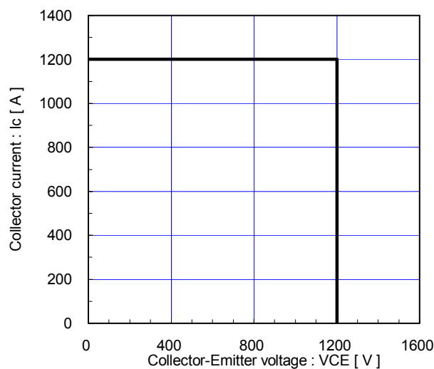
Reverse bias safe operating area (max.) +V_{GE}=15V, -V_{GE} \le 15V, R_G \ge 1.1\Omega, T_J \le 125^\circ C
