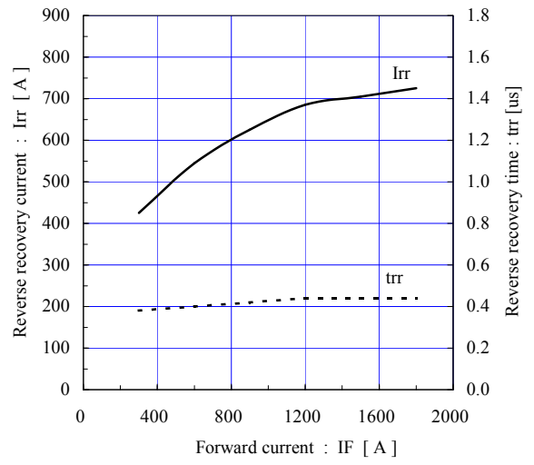
Reverse recovery characteristics (typ.) Vcc=600V, VGE=±15V, Rg=3.3Ω, Tj=125°C
