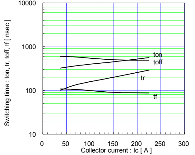
Switching time vs. Collector current (typ.) V_{cc}=600V, V_{GE}=\pm 15V, R_G=4.7\Omega, T_j=125^\circ C
