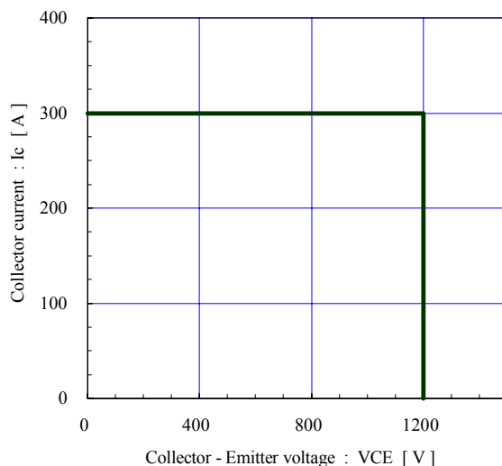
Reverse bias safe operating area (max.) +V_{GE}=15V, -V_{GE} \le 15V, R_g \ge 2.2\Omega, T_j \le 125^\circ C
