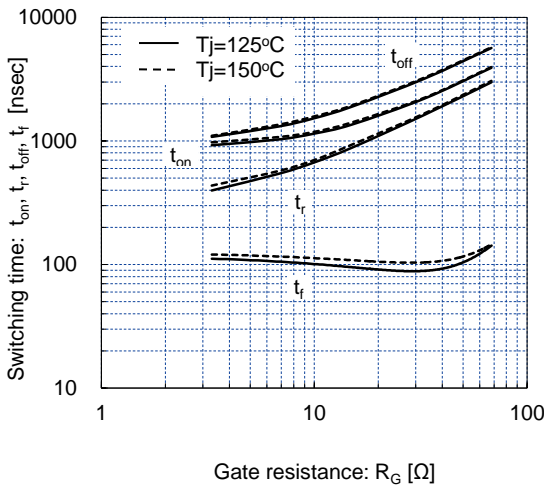
Switching time vs. Gate resistance (typ.) V_{cc}=900V, I_c=225A, V_{GE}=\pm 15V, T_j=125^\circ C, 150^\circ C
