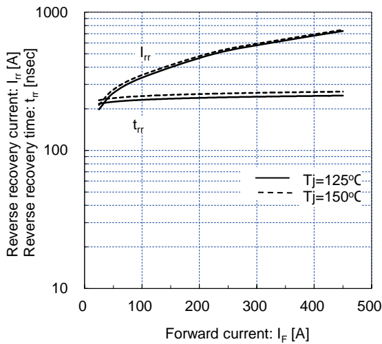
Reverse Recovery Characteristics (typ.) V_{CC}=900\text{V} , V_{GE}=\pm 15\text{V} , R_g=6.8\Omega , T_j=125^\circ\text{C}, 150^\circ\text{C}
