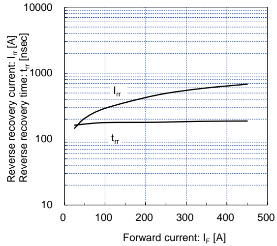
Reverse recovery characteristics (typ.) V_{CC}=900\text{V} , V_{GE}=\pm 15\text{V} , R_g=6.8\Omega , T_j=25^\circ\text{C}
