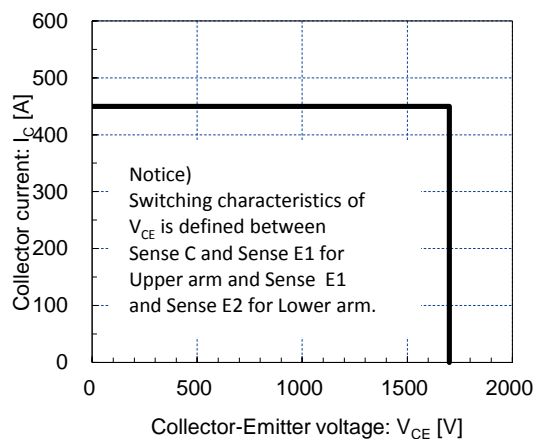
Reverse bias safe operating area (max.) +V_{GE}=15V, -V_{GE}=15V, R_g=6.8\Omega, T_j=150^\circ C
