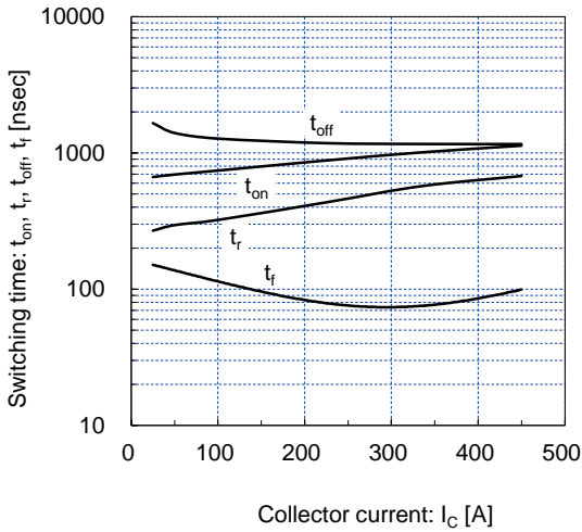
Switching time vs. Collector current (typ.) V_{cc}=900V, V_{GE}=\pm 15V, R_g=6.8\Omega, T_j=25^\circ C
