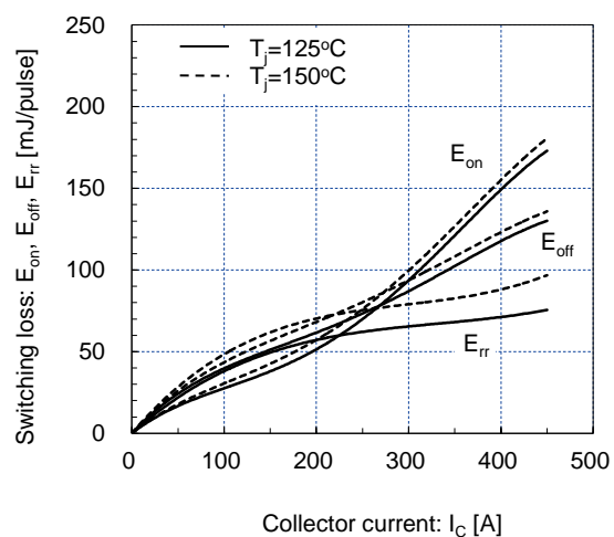
Switching loss vs. Collector current (typ.) V_{cc}=900V, V_{GE}=\pm 15V, R_g=6.8\Omega, T_j=125^\circ C, 150^\circ C
