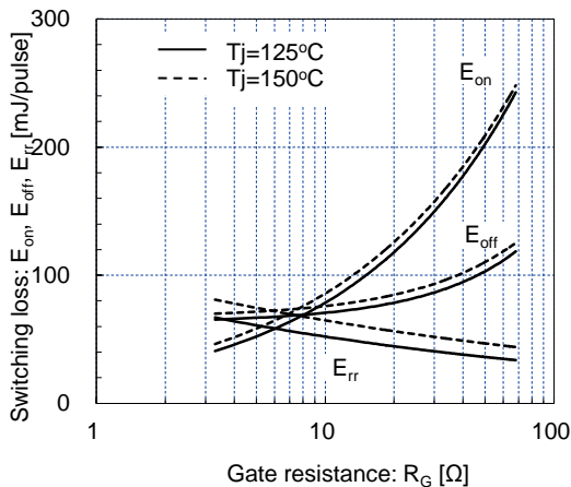
Switching loss vs. Gate resistance (typ.) V_{cc}=900V, I_c=225A, V_{GE}=\pm 15V, T_j=125^\circ C, 150^\circ C
