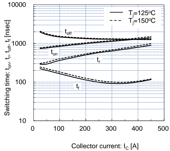
Switching time vs. Collector current (typ.) V_{cc}=900V, V_{GE}=\pm 15V, R_g=6.8\Omega, T_j=125^\circ C, 150^\circ C
