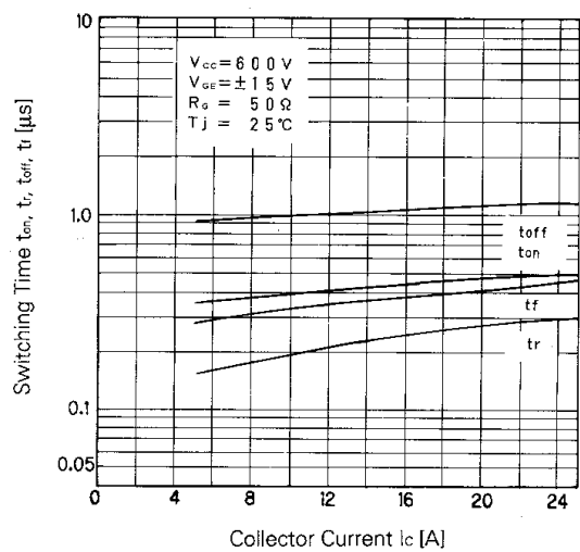
Switching Time
