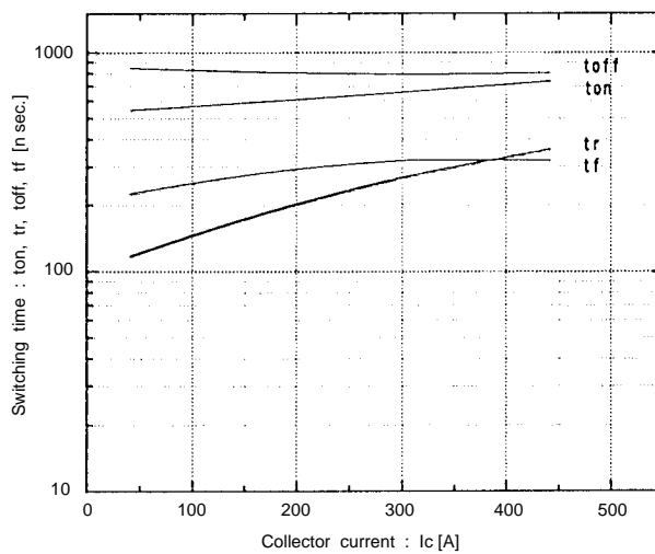
Switching time vs. Collector current V cc =300V, R G =6.8 ohm, V GE =±15V, T j =125°C
