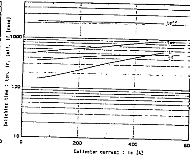
Switching time vs. Collector current Vcc=700V, Rθ=1.2Ω, VGE=15V/-5V, Tj=135°C
