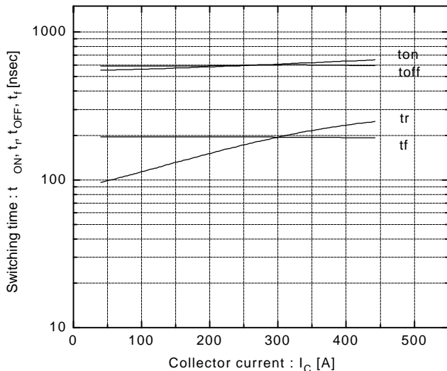
Switching time vs. Collector current V_{CC}=300\text{V}, R_G=6.8\Omega, V_{GE}=\pm 15\text{V}, T_j=25^\circ\text{C}
