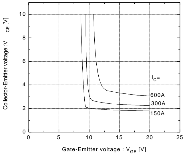
Collector-Emittor vs. Gate-Emittor voltage T_j=25^\circ\text{C}
