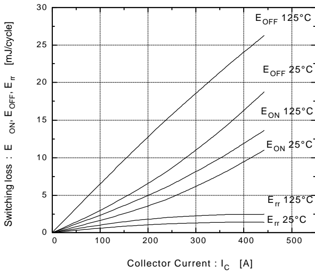
Switching loss vs. Collector current V_{CC}=300V, R_G=6.8\Omega, V_{GE}=\pm 15V
