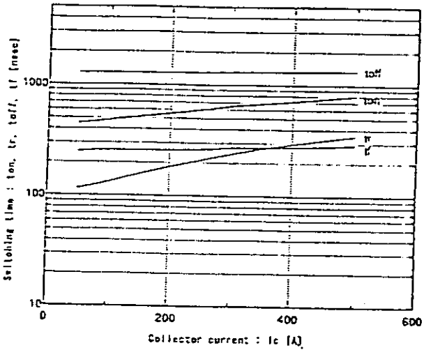
Switching time vs. Collector current Vcc=700V, R6=1.2Ω, VGE=15V/-5V, Tj=25°C
