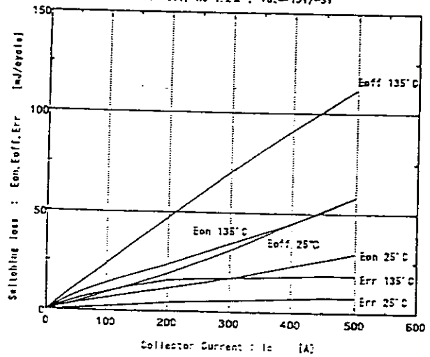
Switching loss vs. Collector current Vcc=700V, R6=1.2Ω, VGE=15V/-5V
