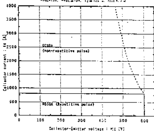
Reversed biased safe operating area +V_{CE} \pm 15V , -V_{GE} \pm 15V , T_J=125^\circ C , R_{th(j-c)}=4.7^\circ C
