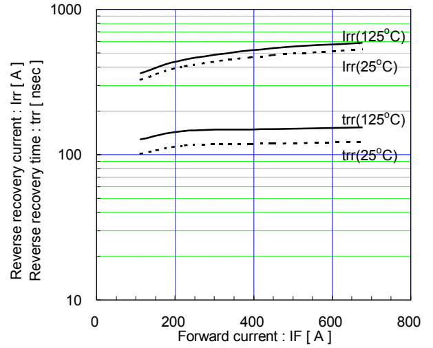
Reverse recovery characteristics (typ.) Vcc=600V, VGE=±15V, RG=0.68Ω
