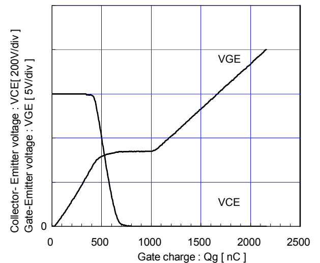
Dynamic Gate charge (typ.) Vcc=600V, Ic=450A, Tj=25°C
