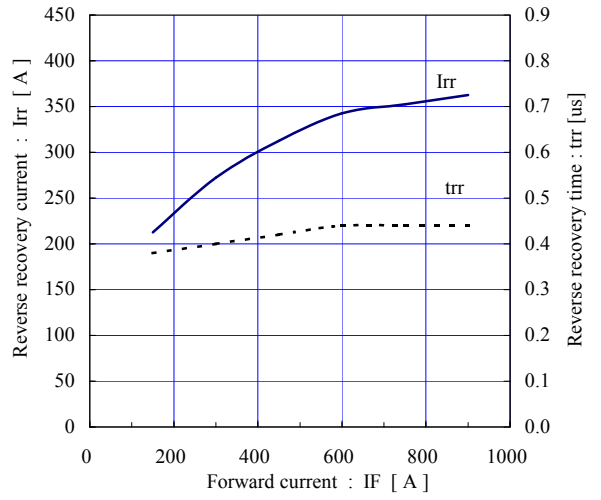
Reverse recovery characteristics (typ.) Vcc=600V, VGE=±15V, Rg=6.8Ω, Tj=125°C
