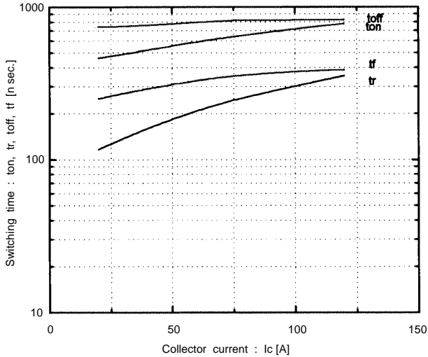
Switching time vs. Collector current V CC =600V, R G =16 ohm, V GE =±15V, T J =25°C
