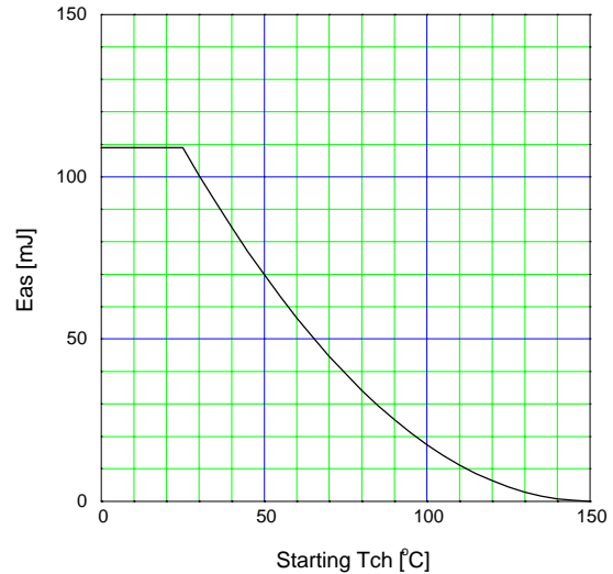
Avalanche energy derating E_{as}=f(\text{starting } T_{ch}):V_{cc}=80V, I_{AV}=4A
