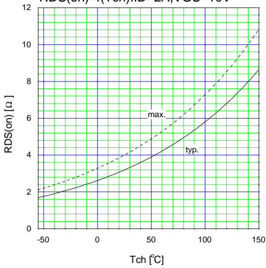
Drain-source on-state resistance R_{DS(on)}=f(T_{ch}):I_D=2A, V_{GS}=10V
