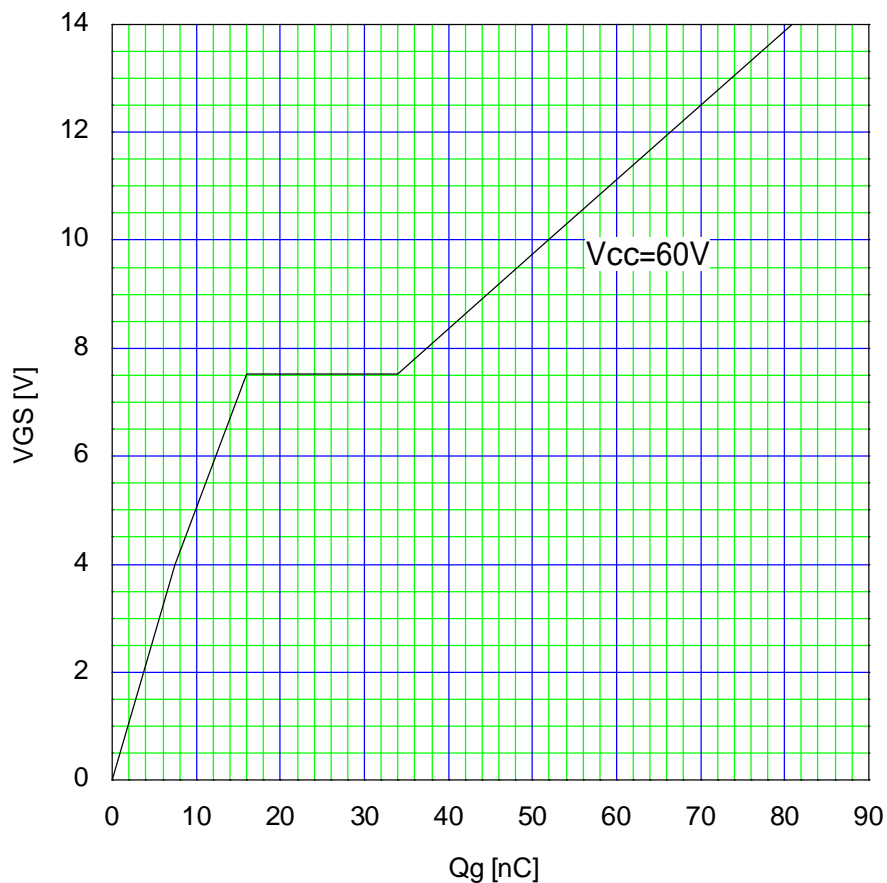
Typical Gate Charge Characteristics V_{GS} = f(Q_g) : I_D = 67A, T_{ch} = 25\text{ °C}
