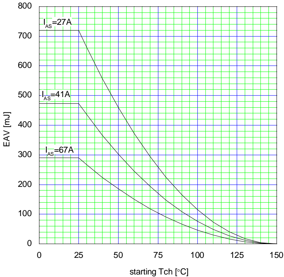
Maximum Avalanche Energy vs. starting Tch E(AV)=f(\text{starting } Tch): V_{CC}=48V, I(AV) \leq 67A
