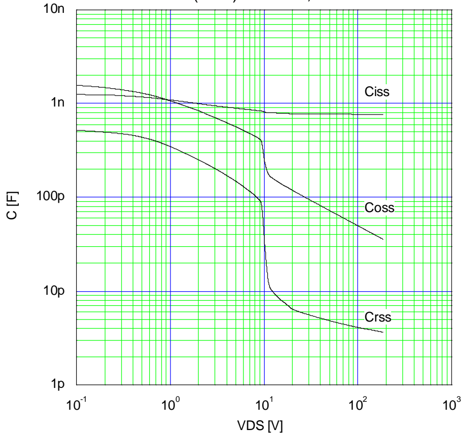
Typical Capacitance C=f(V_{DS}):V_{GS}=0V, f=1MHz
