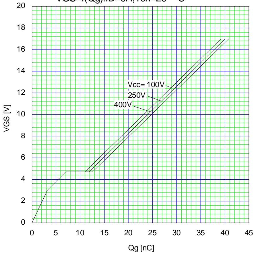
Typical Gate Charge Characteristics V_{GS} = f(Q_g) : I_D = 9A, T_{ch} = 25\text{ }^\circ\text{C}
