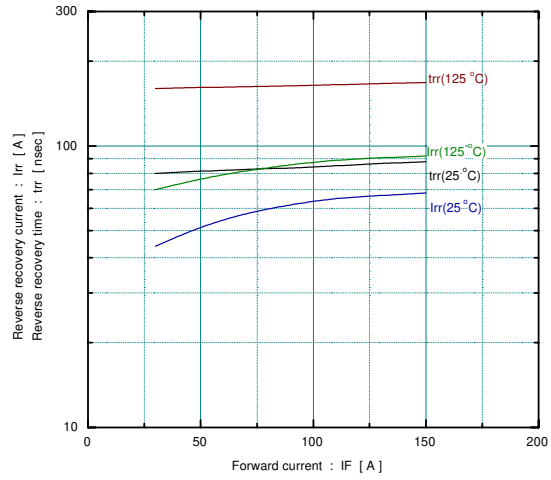
Reverse recovery characteristics (typ.) Vcc=600V, VGE=±15V, Rg=12Ω
