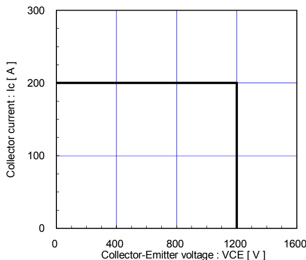
Reverse bias safe operating area (max.) +V_{GE}=15V, -V_{GE} \le 15V, R_G \ge 5.6\Omega, T_J \le 125^\circ C
