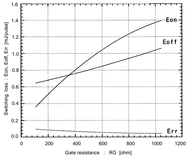
Switching loss vs. Gate resistance V_{cc}=300V, I_c=10A, V_{GE}=\pm 15V, T_J=125^\circ\text{C}
