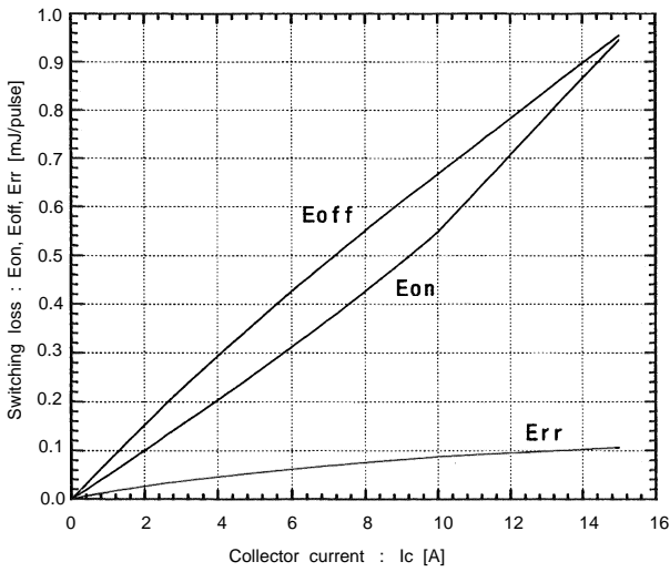
Switching loss vs. Collector current V_{cc}=300V, R_G=220\ \text{ohm}, V_{GE}=\pm 15V, T_J=125^\circ\text{C}
