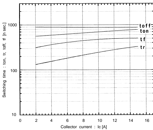
Switching time vs. Collector current V CC =300V, R G =220 ohm, V GE =±15V, T J =125°C
