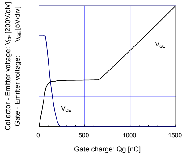
[ Inverter ] Dynamic gate charge (typ.) V_{CC} = 600V , I_c = 150A , T_j = 25^\circ\text{C}
