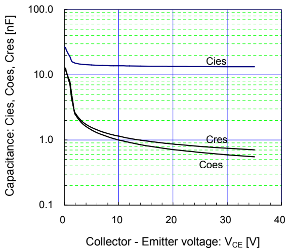
[ Inverter ] Capacitance vs. Collector-Emitter voltage (typ.) V_{GE} = 0V , f = 1\text{MHz} , T_j = 25^\circ\text{C}
