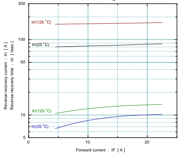
Reverse recovery characteristics (typ.) Vcc=600V, VGE=±15V, Rg=82Ω
