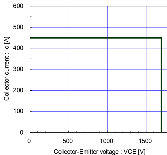
Reverse bias safe operating area (max.) +V_{GE}=15V, -V_{GE} \le 15V, R_g \ge 2.2\Omega, T_j \le 125^\circ C Stray inductance \le 100nH
