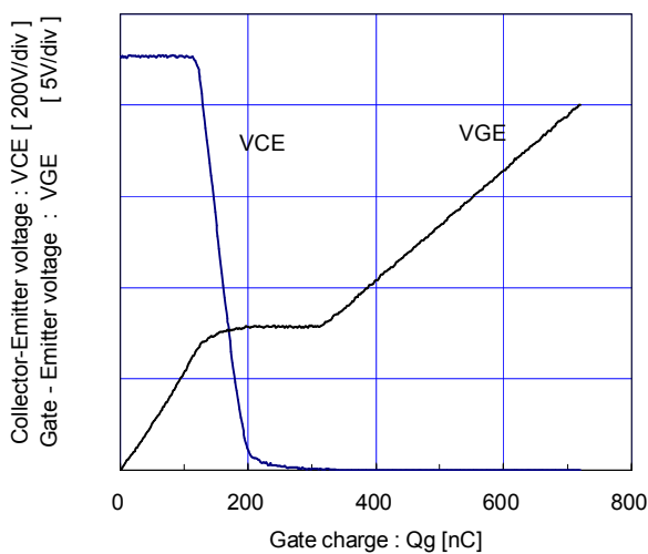
Dynamic Gate charge (typ.) Vcc=900V, Ic=225A, Tj= 25°C
