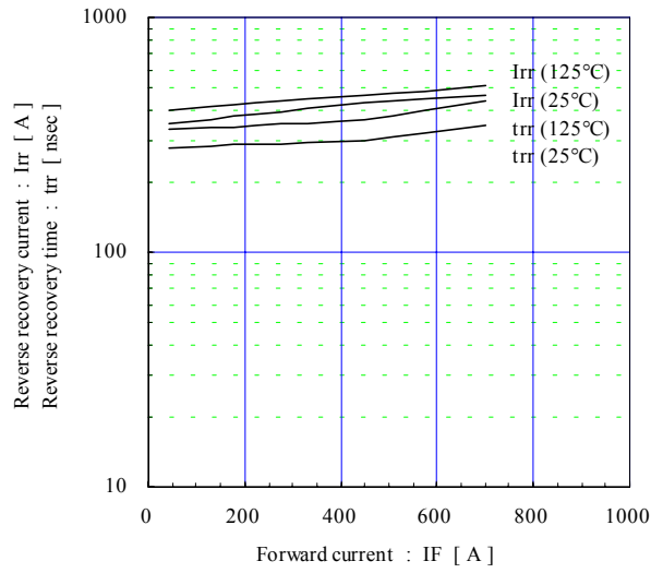
Reverse recovery characteristics (typ.) V_{cc}=900\text{V} , V_{GE}=\pm 15\text{V} , R_g=1.1\Omega
