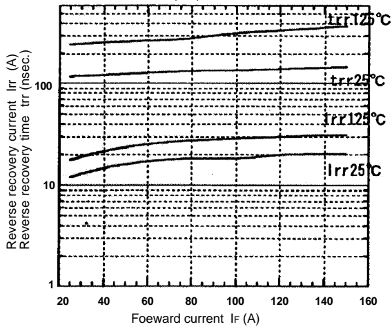
Reverse recovery characteristics t_{rr}, I_{rr}, \text{ vs. } I_F
