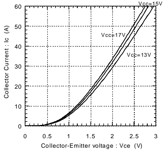
Collector current vs. Collector-Emittor voltage T j =125°C(Terminal)
