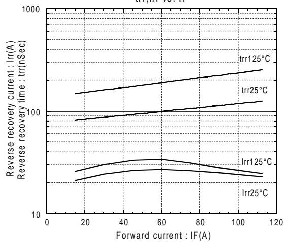
Reverse recovery characteristics trr, I rr vs. I F
