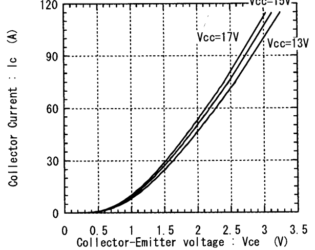
Collector current vs. Collector-Emitter voltage Tj=125°C (Terminal)
