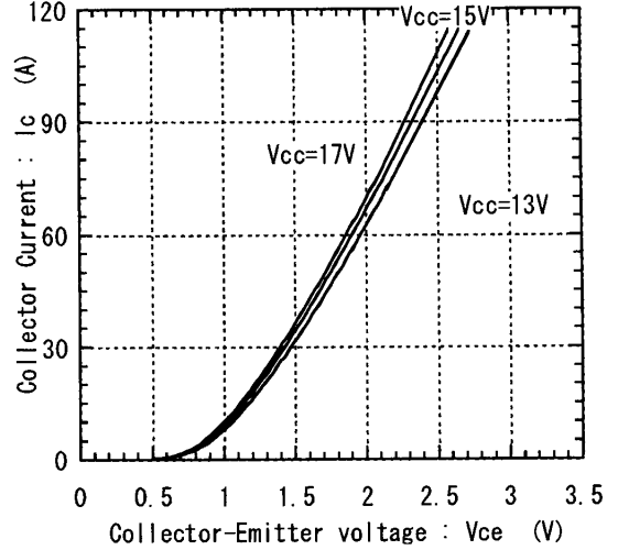
Collector current vs. Collector-Emitter voltage Tj=25°C (Terminal)
