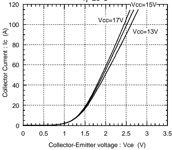
Collector current vs. Collector-Emmitter voltage Tj=25°C
