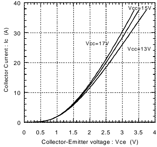
Collector current vs. Collector-Emmitter voltage (typ.) Tj=125°C
