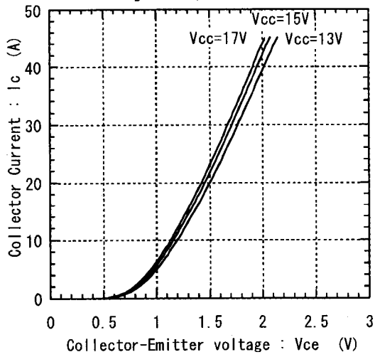
Collector current vs. Collector-Emittor voltage T_j=25^\circ\text{C} (Terminal)
