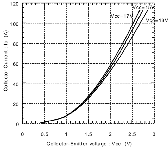
Collector current vs. Collector-Emitter voltage Tj=125°C(Chip)
