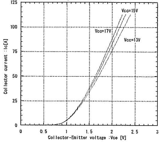
Collector current vs. Collector-Emittor voltage (typ.) T j =25°C (Terminal)
