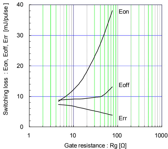
[ Inverter ] Switching loss vs. Gate resistance (typ.) Vcc=600V, Ic=100A, VGE=±15V, Tj= 125°C
