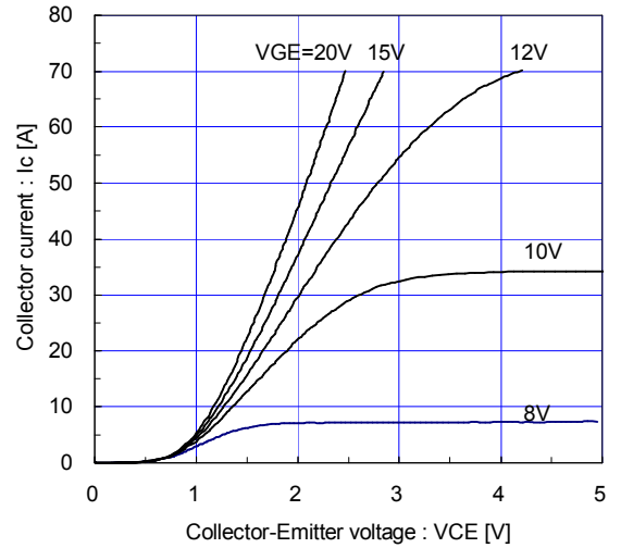
[ Brake ] Collector current vs. Collector-Emmitter voltage (typ.) T_j = 125^\circ\text{C} / chip
