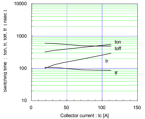
[ Inverter ] Switching time vs. Collector current (typ.) Vcc=600V, VGE=±15V, Rg=9.1Ω, Tj=125°C
