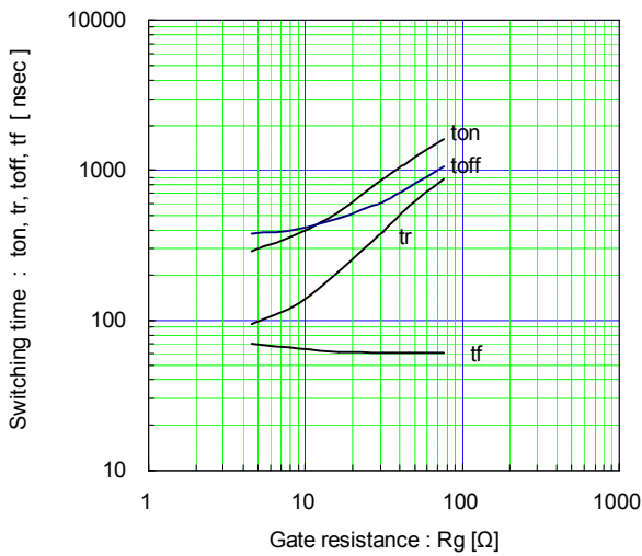
[ Inverter ] Switching time vs. Gate resistance (typ.) Vcc=600V, Ic=100A, VGE=±15V, Tj= 25°C
