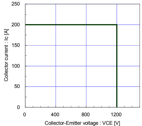
[ Inverter ] Reverse bias safe operating area (max.) +VGE=15V, -VGE ≤ 15V, RG ≥ 9.1Ω, Tj ≤ 125°C
