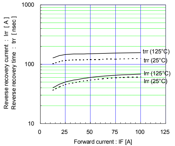
[ Inverter ] Reverse recovery characteristics (typ.) V_{cc}=600V, V_{GE}=\pm 15V, R_g=9.1\Omega
