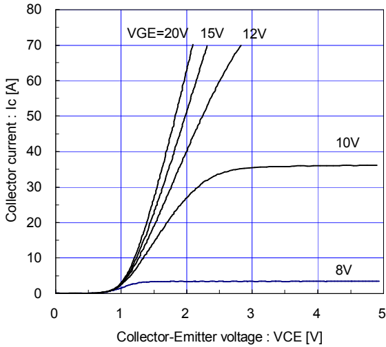
[ Brake ] Collector current vs. Collector-Emmitter voltage (typ.) T_j = 25^\circ\text{C} / chip
