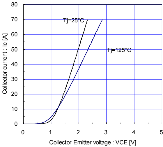
[ Brake ] Collector current vs. Collector-Emmitter voltage (typ.) V_{GE} = 15\text{V} / chip
