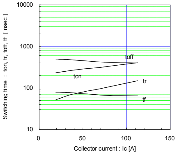
[ Inverter ] Switching time vs. Collector current (typ.) Vcc=600V, VGE=±15V, Rg=9.1Ω, Tj= 25°C
