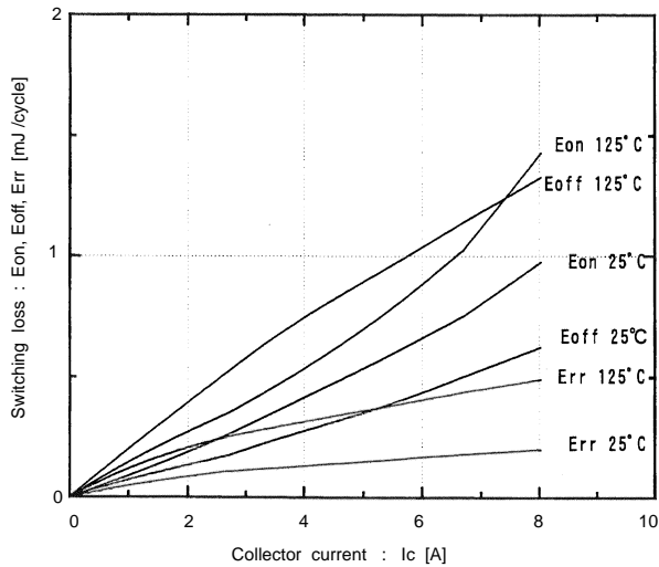
Switching loss vs. Collector current V_{CC}=600V, R_G=120 \Omega, V_{GE}=\pm 15V
