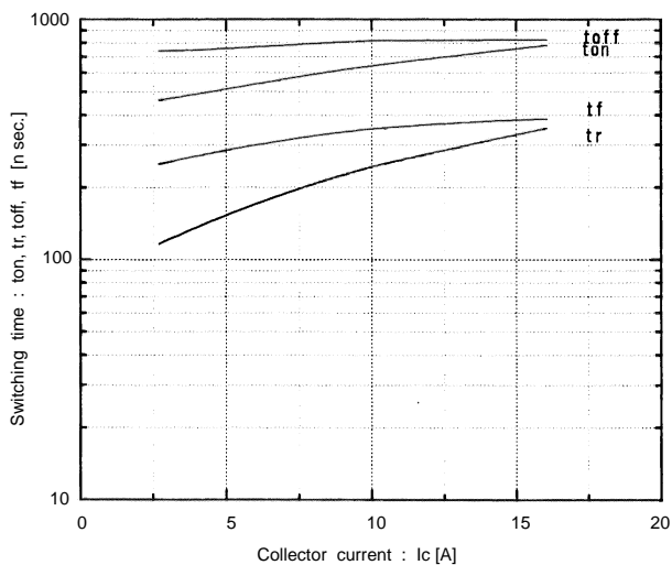
Switching time vs. Collector current V cc =600V, R G =62 ohm, V GE =±15V, T J =25°C
