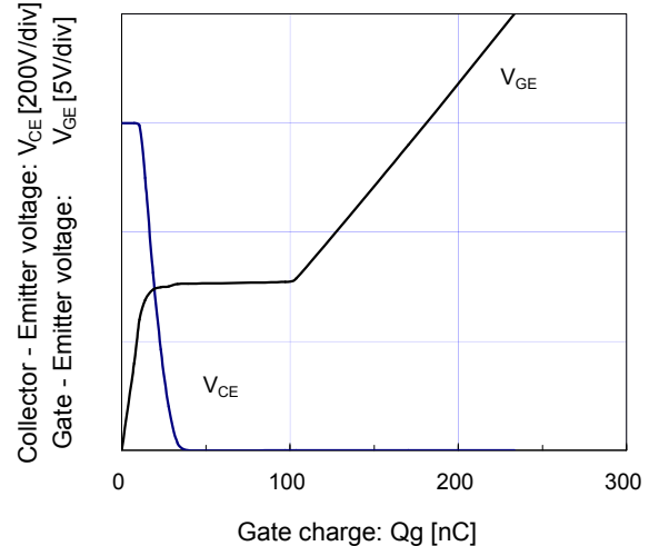
Dynamic gate charge (typ.) Vcc=600V, Ic=25A, Tj= 25°C
