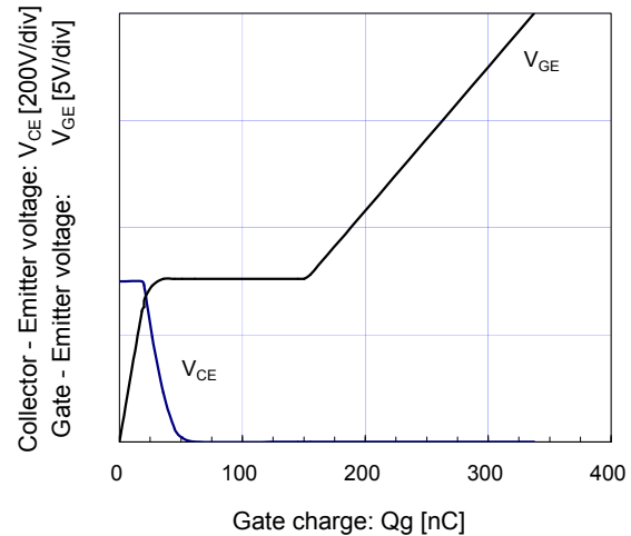
[ Brake ] Dynamic gate charge (typ.) V_{CC} = 300\text{V} , I_c = 75\text{A} , T_j = 25^\circ\text{C}
