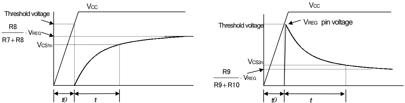
t0: Time from power-on of VCC to reaching unlock voltage of UVLO
