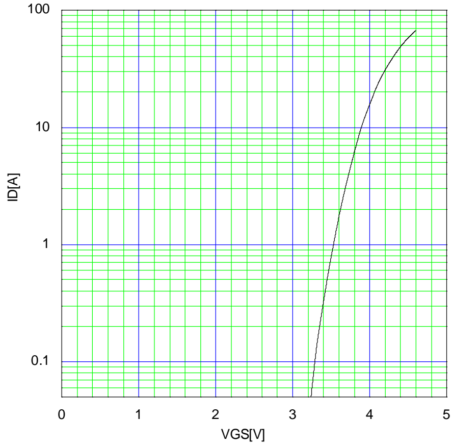
Typical Transfer Characteristic I_D=f(V_{GS}):80\ \mu\text{s pulse test}, V_{DS}=25\text{V}, T_{ch}=25\ \text{°C}
