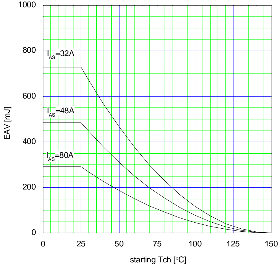
Maximum Avalanche Energy vs. starting Tch E(AV)=f(\text{starting Tch}):V_{CC}=48V, I(AV)\leq 80A
