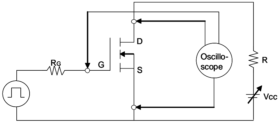
Fig.3 Switching Test circuit
