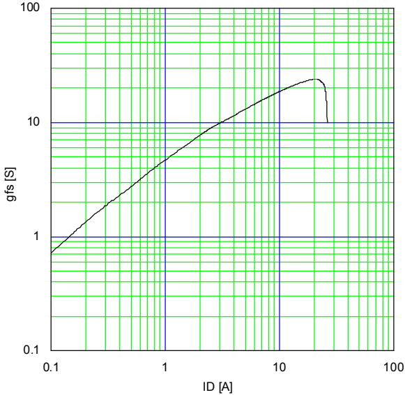
Typical Transconductance
